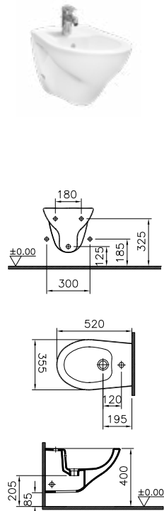
DIANA O100 Wand-Bidet Ausladung 520 mm, (DI000400001)
