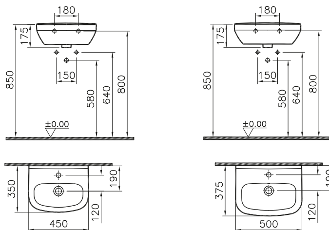
DIANA S100 Handwaschbecken rund 450 x 350 mm, (DI001314...) 110,- € 500 x 375 mm, (DI001316...) 114,- €
