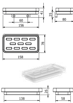
DIANA L100 Kristallseifenschale matt, (DI600063) 44,10 €
