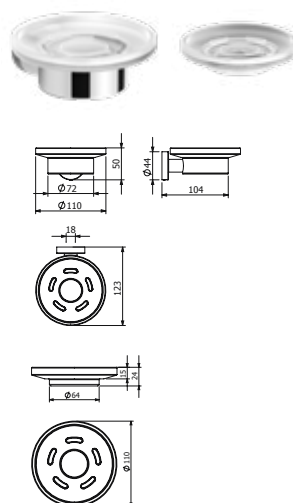
DIANA M200-Neu Wand-Seifenhalter verchromt, (DI602022500) 62,90 € Schwarz matt, (DI602022530) 78,10 €
